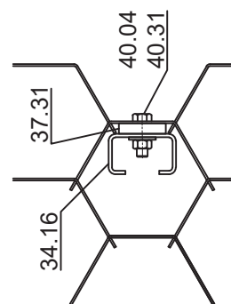
Detail X
