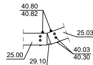
Detail Z
